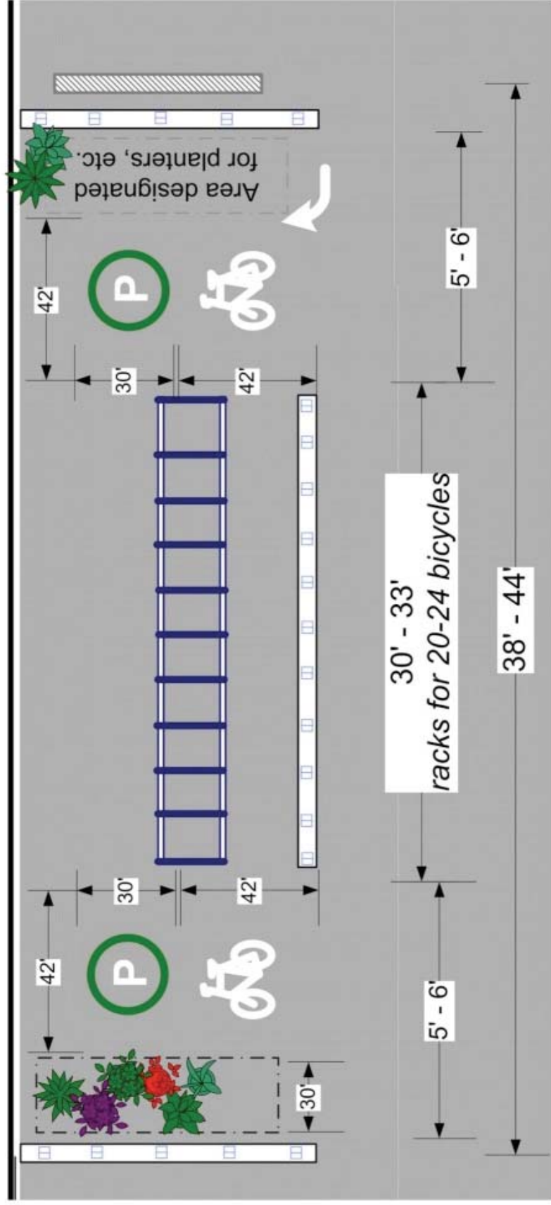
Typical downtown in-street bicycle parking design (Portland Bureau of Transportation)
