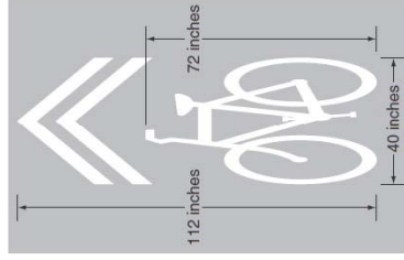
Sharrow (MUTCD 9C-9)
