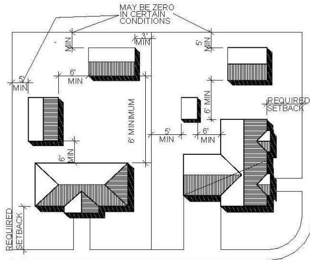
Figure 19.57-A: Accessory Structure Setbacks
